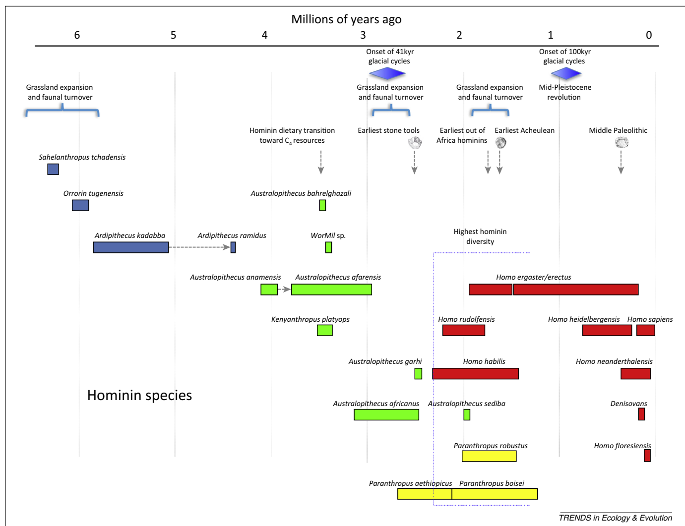
Figure 4. Time range of hominin species, with major climatic, environmental, and cultural developments. At approximately 3.4 million years ago (Mya), there were at least four hominin species in Africa, but so far there is no evidence for their sympatry. Between approximately 2.5 and 1.4 Mya, there is evidence of Homo and Paranthropus species co-occurring (and possibly coexisting) at several sites in the Omo-Turkana Basin of Ethiopia and Kenya. Produced by René Bobe.
