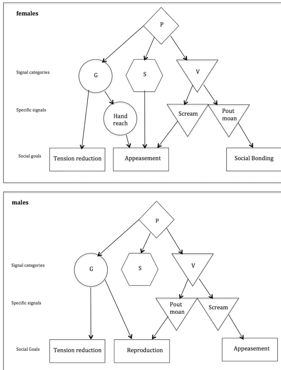
Figure 5. Summary plot of the most likely communicative strategy depending on the social goal of sex and gender of initiator. Arrows represent the most likely scenario based on the result of the statistical models for signal categories and on the descriptive analyses of proportions for specific signals. P = Sexual initiation posture; G = Gesture; S = Sequence; V = Vocalisation.
